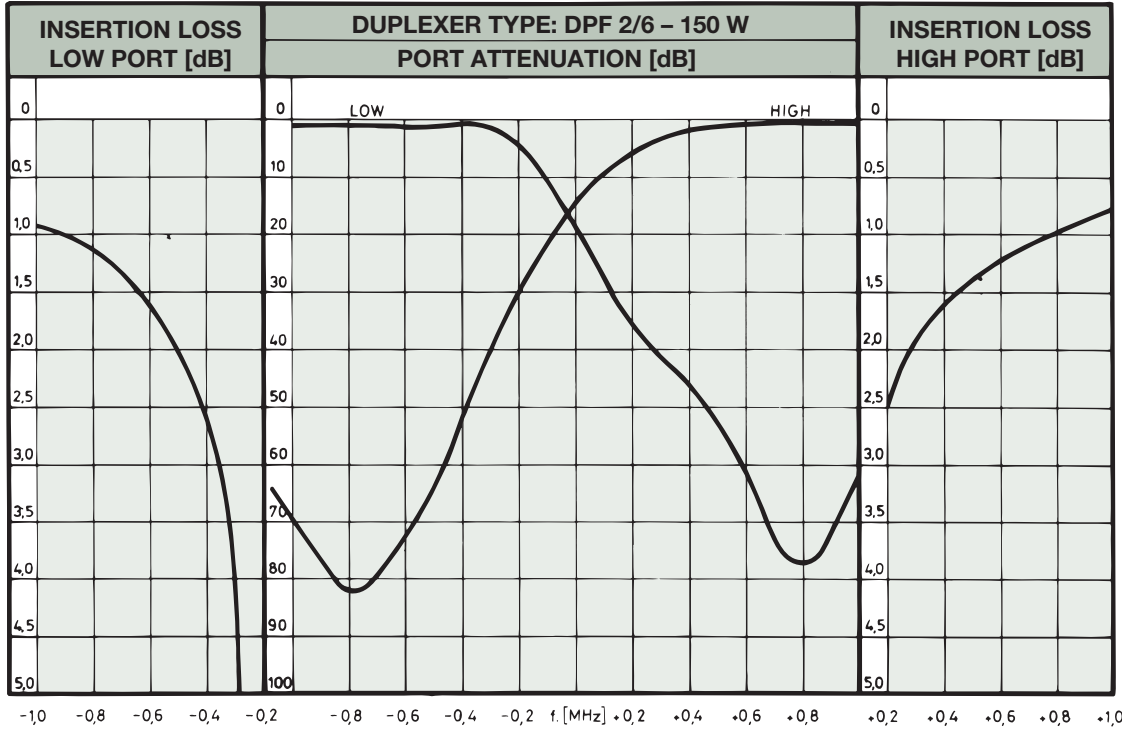
TYPICAL RESPONSE CURVES @ 1.6 MHz DUPLEX SPACING:
