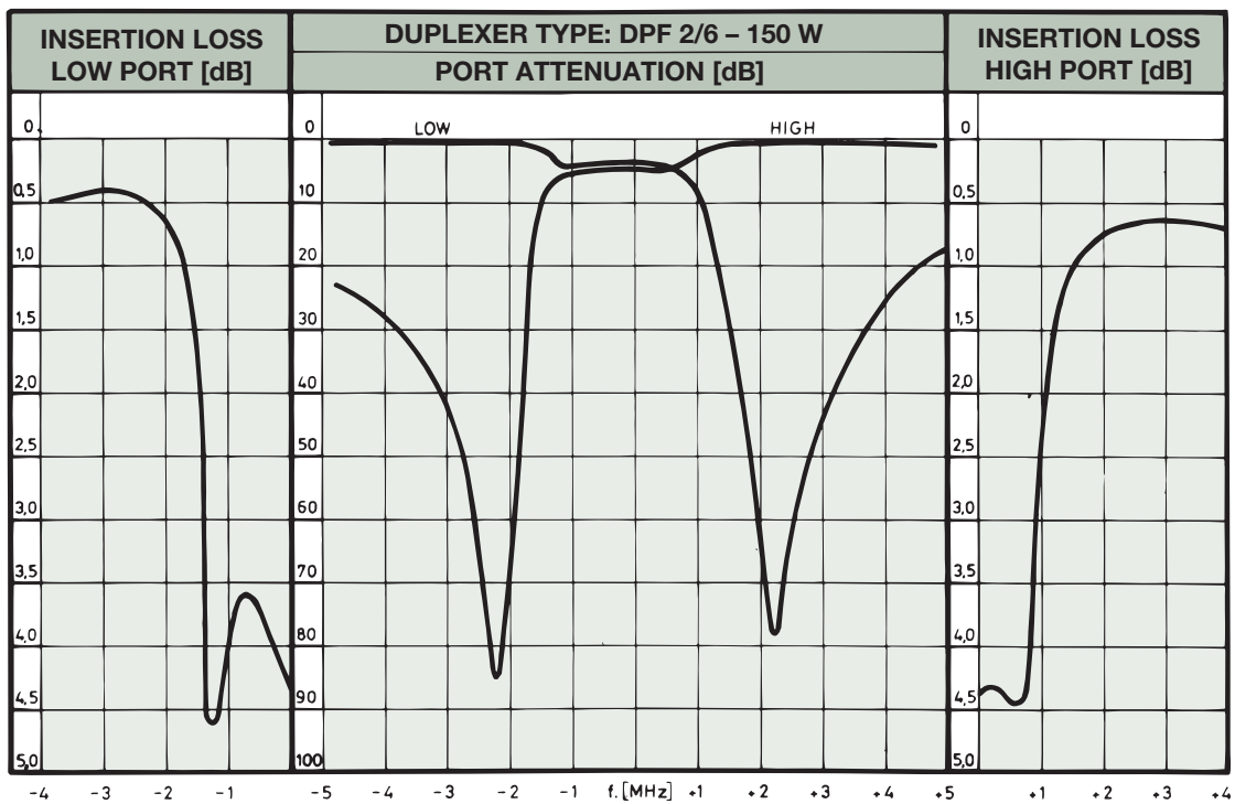
TYPICAL RESPONSE CURVES @ 4.5 MHz DUPLEX SPACING:
