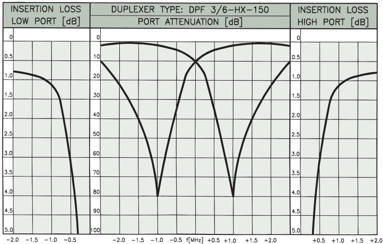
TYPICAL RESPONSE CURVES @ 2 MHz DUPLEX SPACING:
