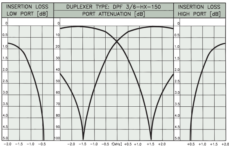
TYPICAL RESPONSE CURVES @ 3 MHz DUPLEX SPACING:
