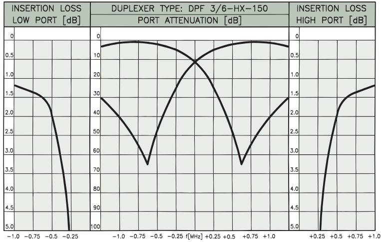
TYPICAL RESPONSE CURVES @ 1.3 MHz DUPLEX SPACING:
