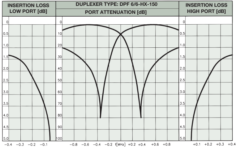
TYPICAL RESPONSE CURVES @ 0.7 MHz DUPLEX SPACING:
