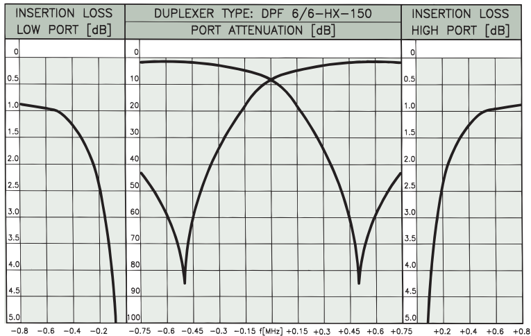
TYPICAL RESPONSE CURVES @ 1 MHz DUPLEX SPACING:
