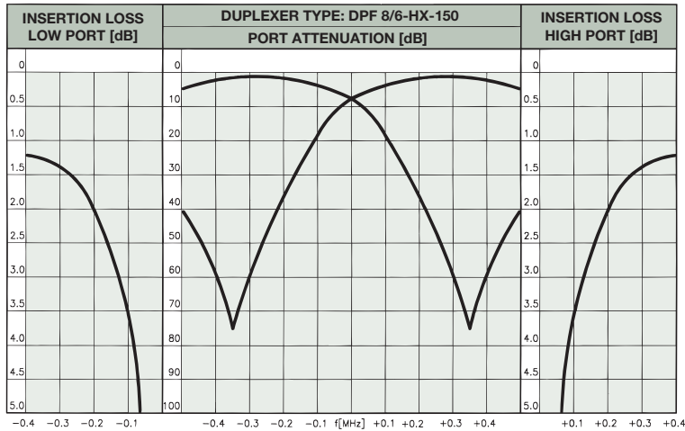
TYPICAL RESPONSE CURVES @ 0.75 MHz DUPLEX SPACING:
