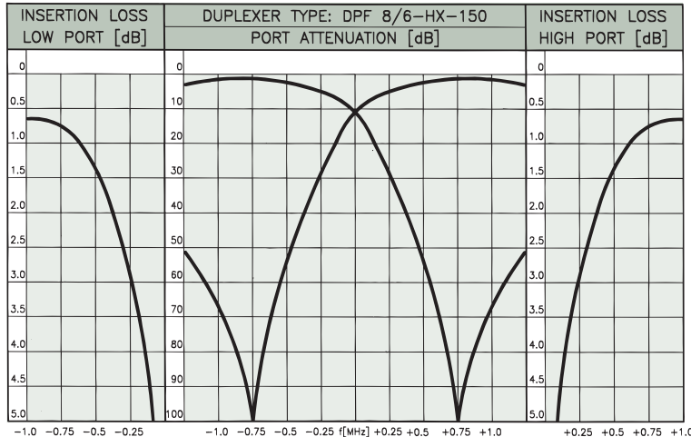
TYPICAL RESPONSE CURVES @ 1.5 MHz DUPLEX SPACING:
