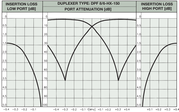
TYPICAL RESPONSE CURVES @ 0.6 MHz DUPLEX SPACING:
