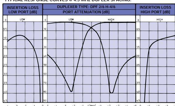
TYPICAL RESPONSE CURVES @ 4.5 MHz DUPLEX SPACING:
