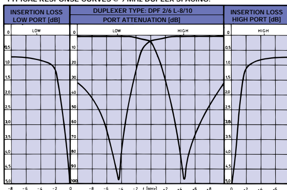
TYPICAL RESPONSE CURVES @ 9 MHz DUPLEX SPACING:
