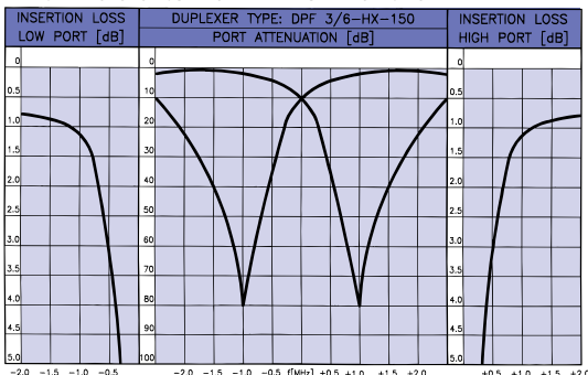
TYPICAL RESPONSE CURVES @ 2 MHz DUPLEX SPACING:
