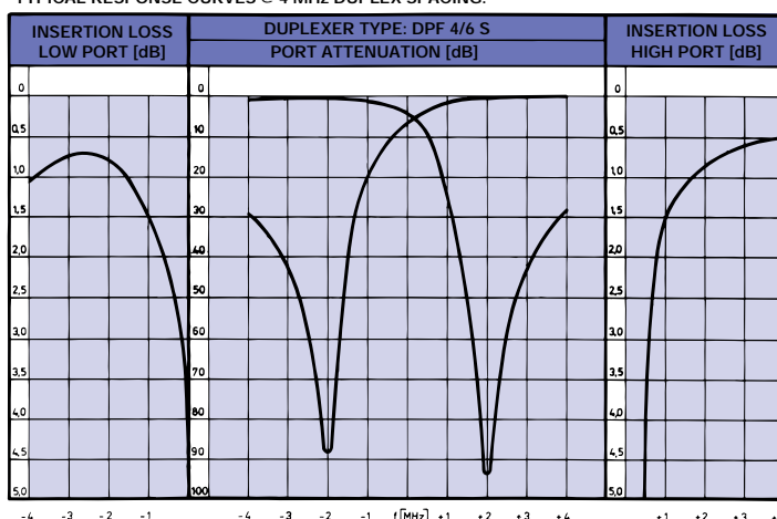
TYPICAL RESPONSE CURVES @ 4 MHz DUPLEX SPACING:
