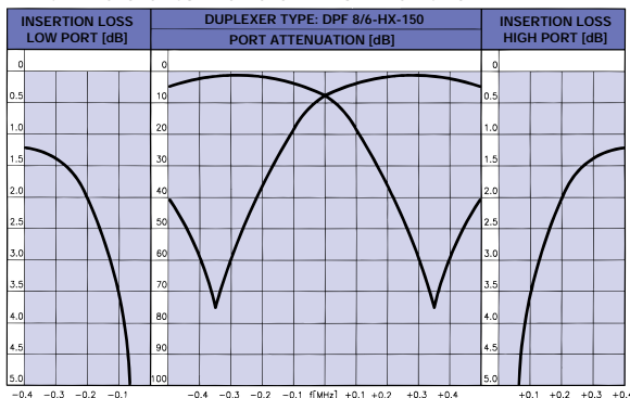
TYPICAL RESPONSE CURVES @ 0.75 MHz DUPLEX SPACING:
